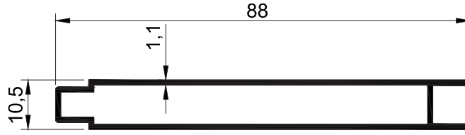
T17 - 0.655 kg/mt
