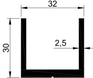
T53 - 0.620 kg/mt
