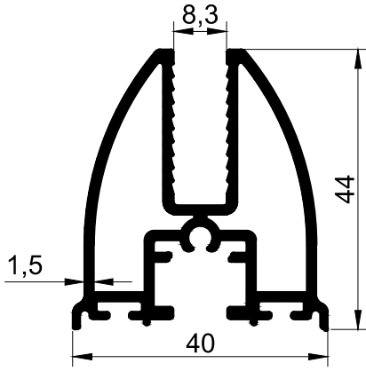
T 2513 0.995 kg/m
