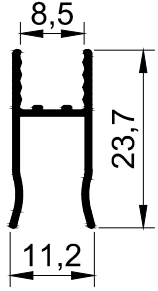
T 934 -0.130 kg/m
