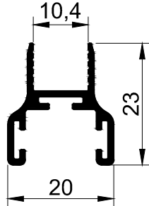
T 598-0.242 kg/m
