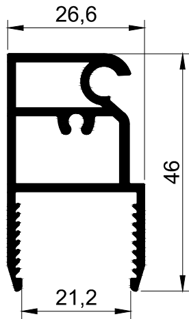
T1262 - 0.735 kg/m
