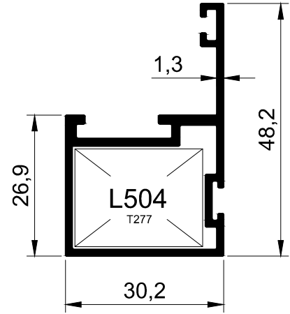
T1258 - 0.585 kg/m
