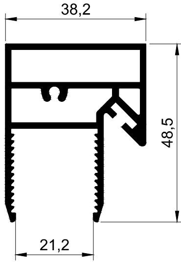
T1255 - 1.007 kg/m
