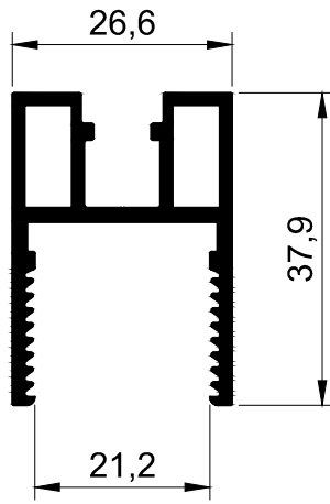
T1257 - 0.647 kg/m
