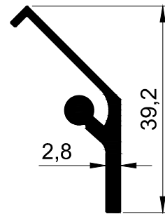
T1263 - 0.356 kg/m
