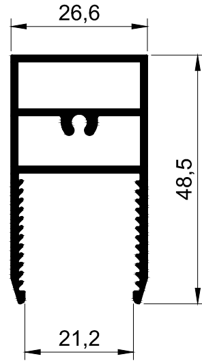
T1254 - 0.690 kg/m
