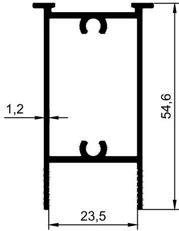
T1684 -0.650 kg/m
