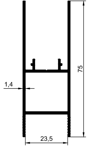
T1683 -0.805 kg/m
