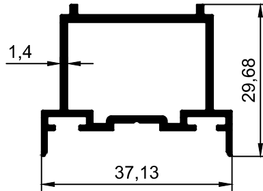
T1681 -0.510 kg/m
