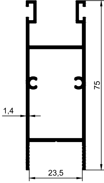
T1682 -0.865 kg/m
