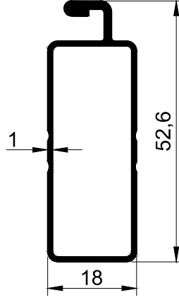
T 1136 - 0.410 kg/m
