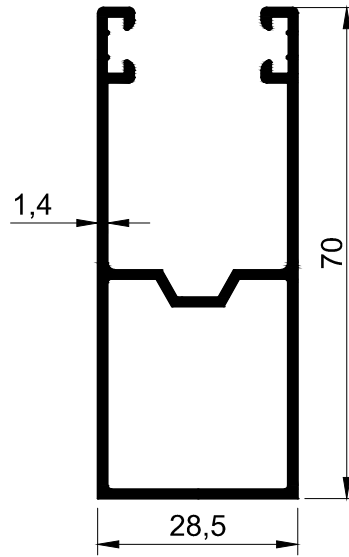
T 816 - 0.830 kg/m
