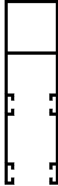
T 2128 - 0.834 kg/m
