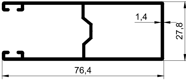
T 2134 - 0.817 kg/m
