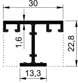
T2051 - 0.336 kg/mt
