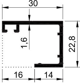
T2050 - 0.307 kg/mt
