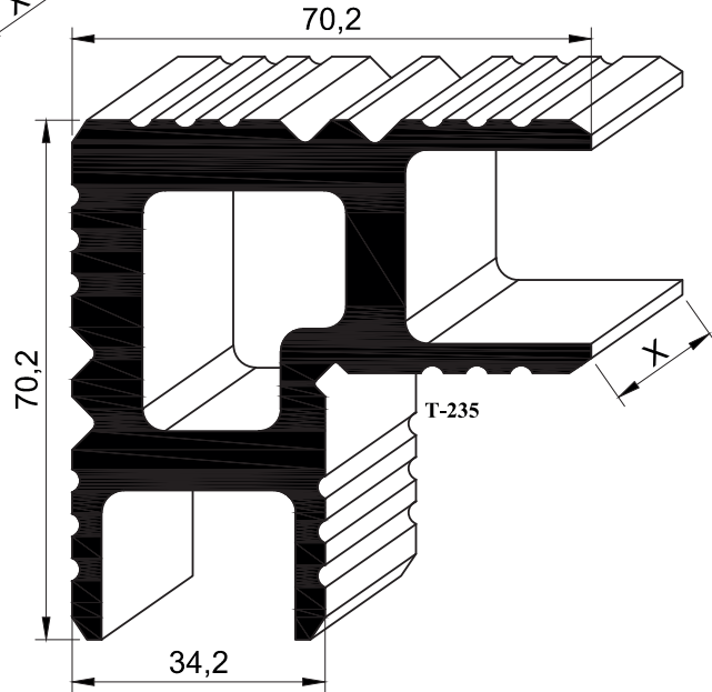
T509 - 4.255 kg/mt
