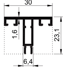
T2049 - 0.345 kg/mt
