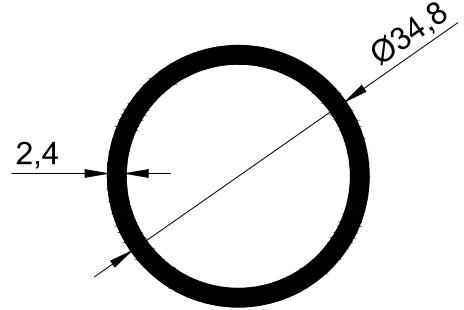
T434-2.4 - 0.670 kg/m
