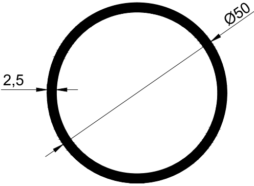
T426-2.5 - 1,050 kg/m
