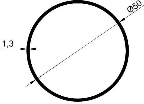
T427-1.3 - 0.545 kg/m
