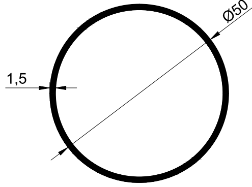
T427-1.5 - 0.625 kg/m
