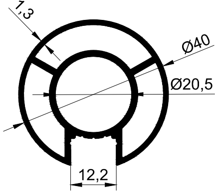
T-2322 - 0.830 kg/m
