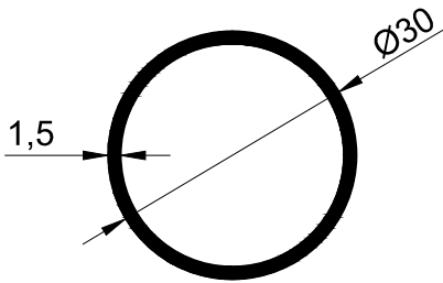
T492-1.7 - 0.380 kg/m
