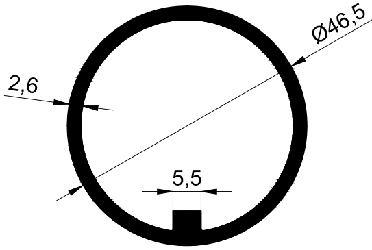
T-2350 - 1.045 kg/m
