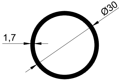
T439-1.7 - 0.412 kg/m
