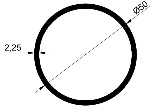
T433-2.25 - 0.921 kg/m
